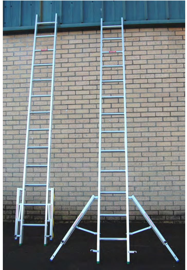
Clow Dual Section Extension Ladder to EN131:Professional
